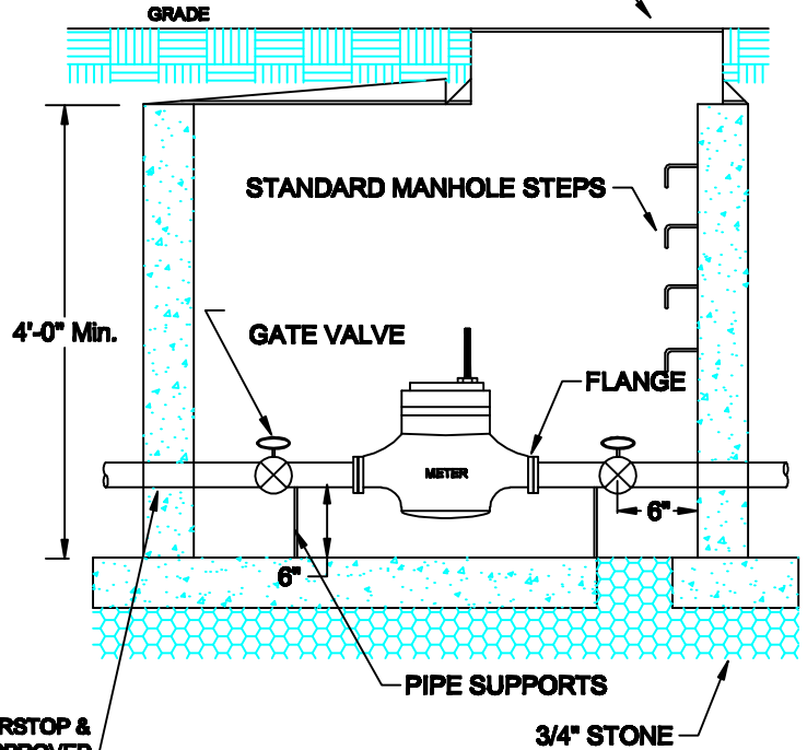
SECTION A
