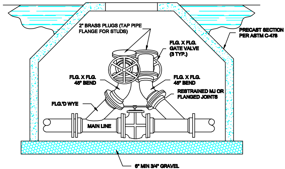
SECTION VIEW
